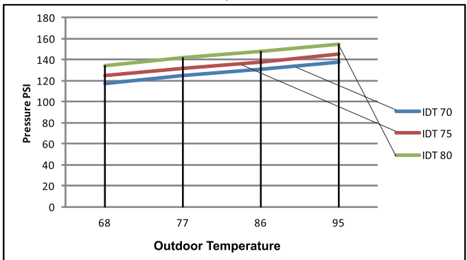
Outdoor Ambient Temperature VS Pressure
