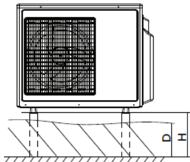
Correct installation
