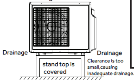
Wrong installation
