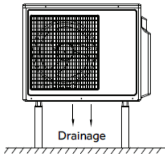
Correct installation
